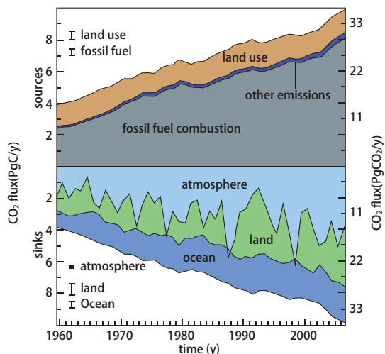
Figure 4: Artificial CO 2 emissions and environmental CO 2 absorption
