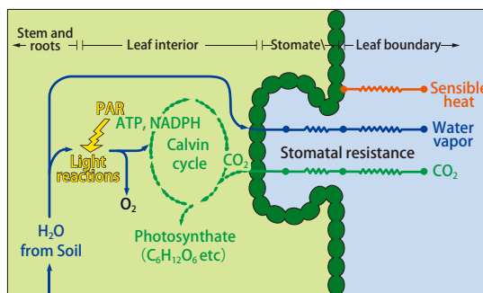
Figure 2: Leaf photosynthesis and stomatic function
